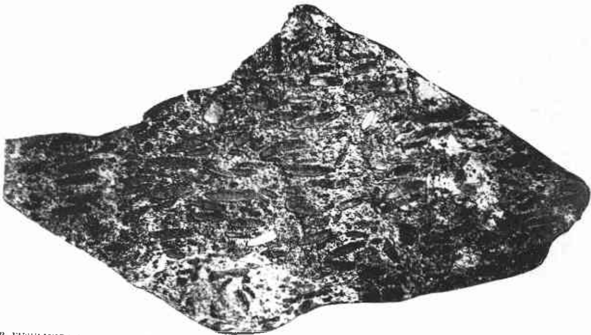
B. FUSULINIDS (PARAFUSULINA SP.) IN SANDSTONE OF BRUSHY CANYON FORMATION, SHOWING TENDENCY TOWARD PARALLEL ORIENTATION.
