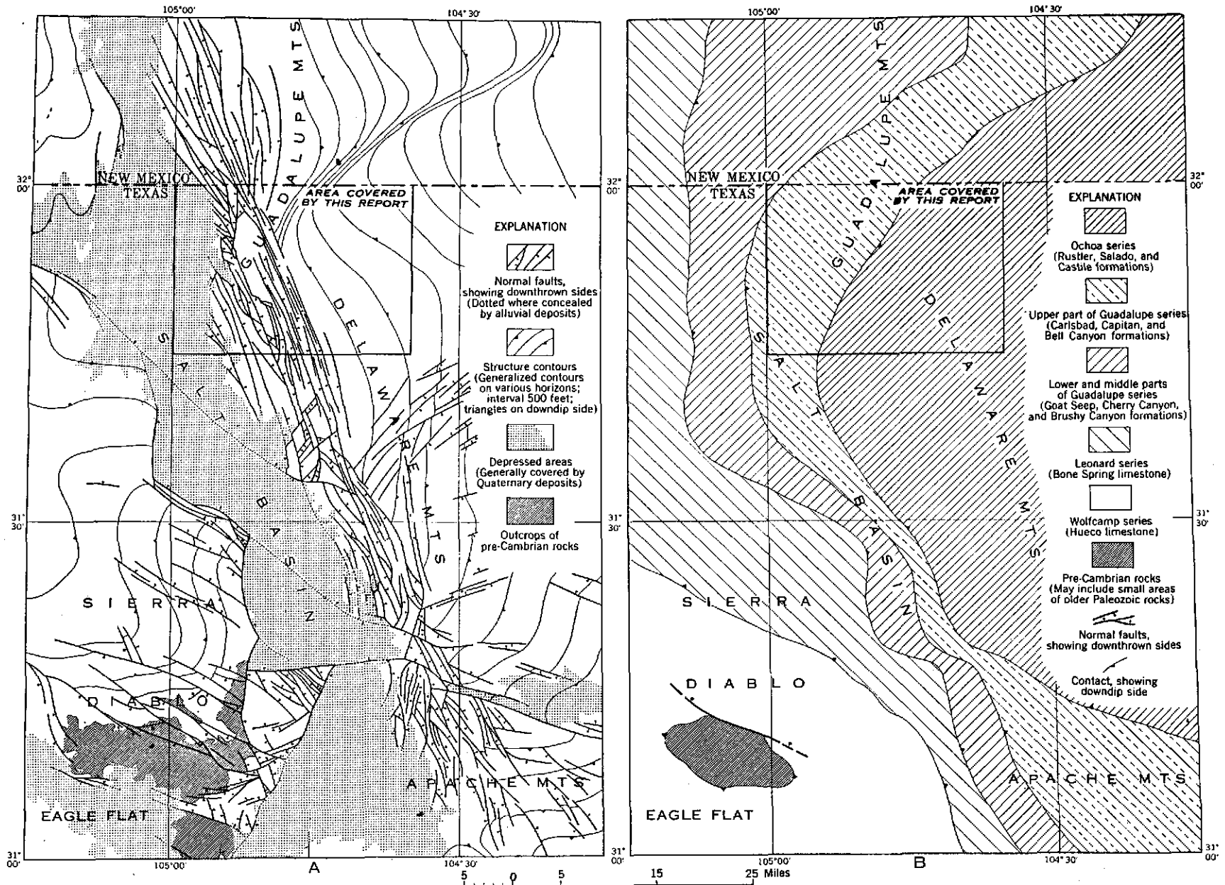
FIGURE 15.—Maps showing tectonic features of Guadalupe Mountains and vicinity during different periods. A, Tectonic features of Cenozoic time; B, Tectonic features of early Mesozoic time, as suggested by paleogeologic map of surface on which Cretaceous was deposited.
