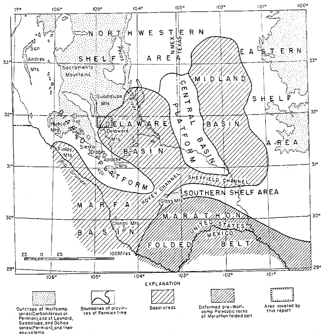
FIGURE 3.—Index map of parts of western Texas and southeastern New Mexico, showing provinces of Permian time.
