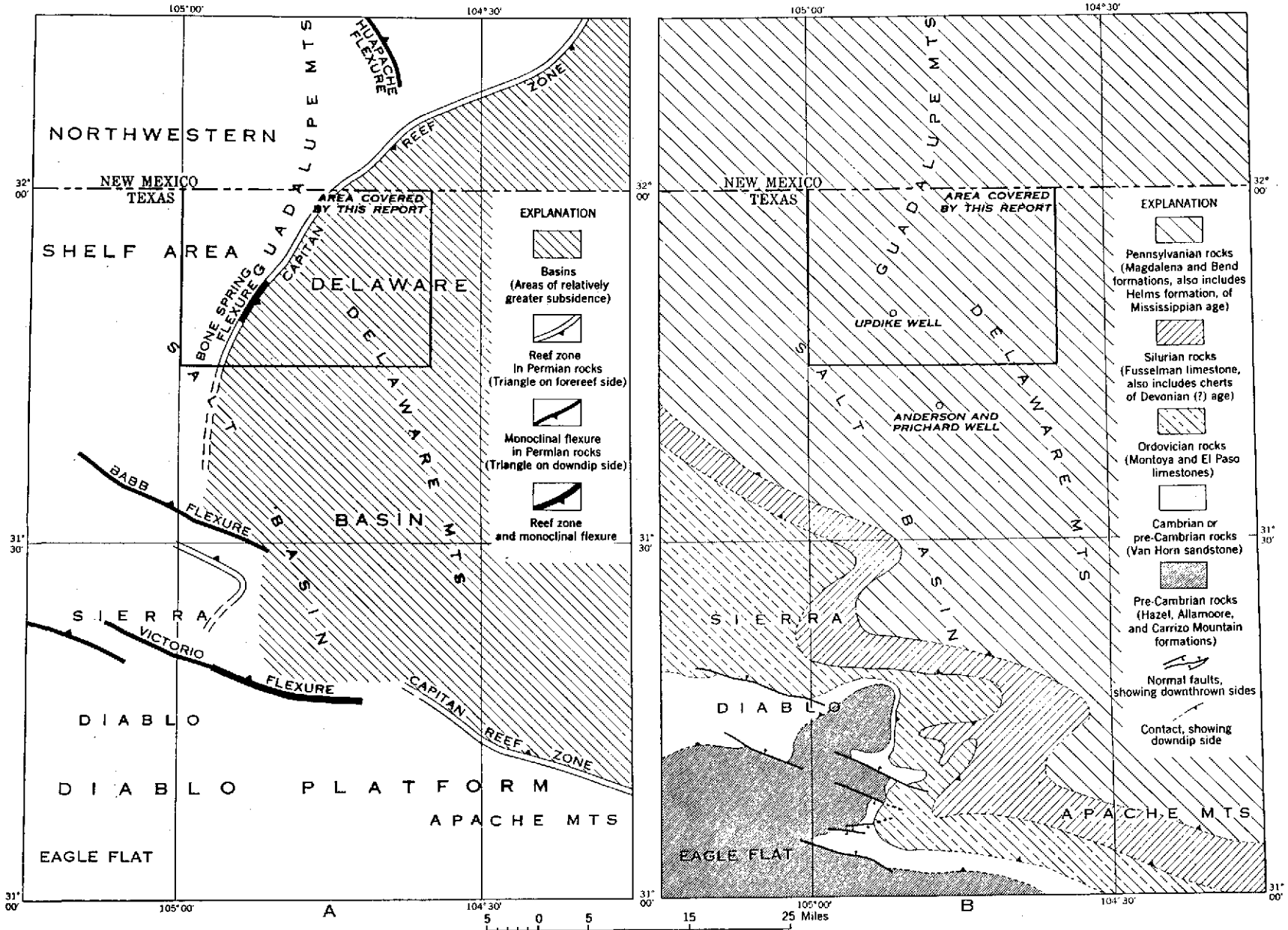
FIGURE 16.—Maps showing tectonic features of Guadalupe Mountains and vicinity during different periods. A, Tectonic features of Permian time; B, Tectonic features of late Carboniferous time, as suggested by paleogeologic map of surface on which Wolfcamp series was deposited.
