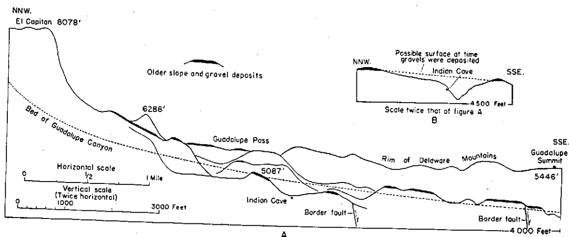
FIGURE 24.—Sections south of El Capitan. A, Projected profiles, showing relation of older slope deposits to present topography; B, Section showing relation of older slope deposits to Indian Cave, which contains late Pleistocene or early Recent fossils.
